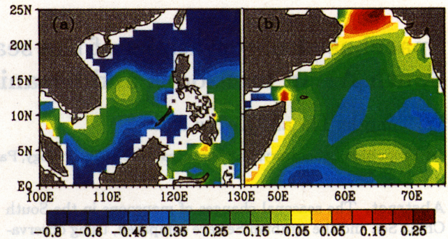
Figure 3. Distribution of correlation coefficients between latent heat flux and sea surface temperature tendency in (a) SCS, and (b) AS.
