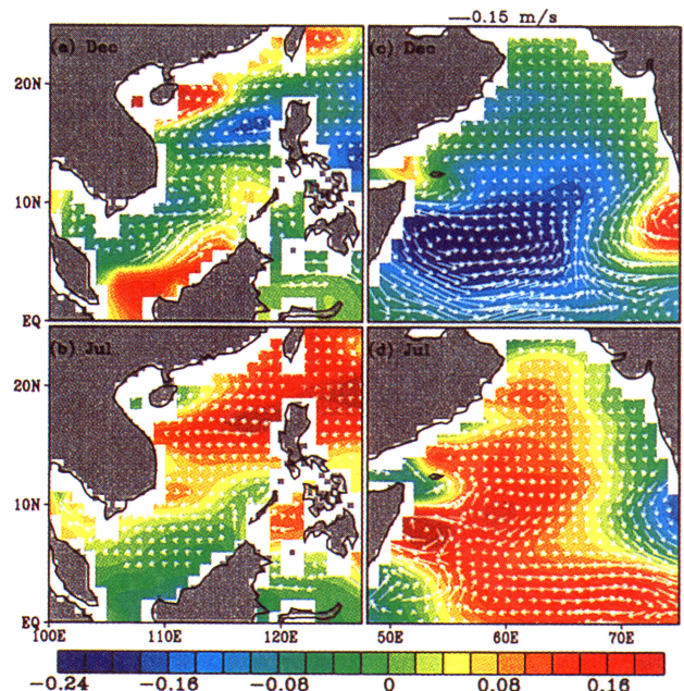
Figure 6. Same as Fig. 5, except for sea level changes (m) and geostrophic currents.
