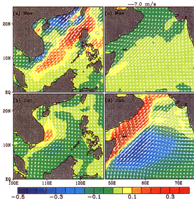
Figure 5. Distribution of curl of wind stress ( 10^{-6} N/m^3 ) and wind vectors in SCS and AS for typical months.
