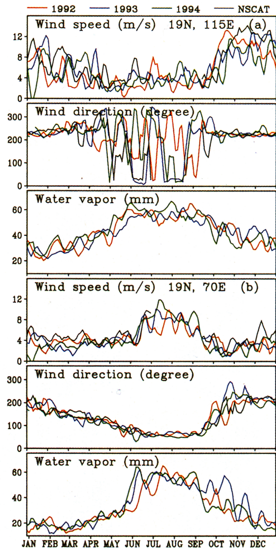
Figure 1. Time series of wind speed, wind direction, and integrated water vapor at (a) 19°N and 115°E in the South China Sea, and (b) 19°N and 70°E in the Arabian Sea. Winds blowing towards the north are represented by 0° in wind direction.
