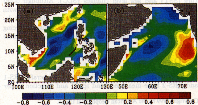
Figure 4. Correlation coefficients between curl of wind stress and sea level changes, with curl of wind stress leading sea level changes by one month, in (a) SCS, and (b) AS.
