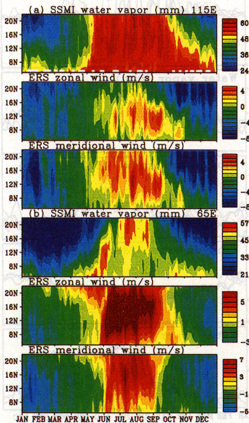
Figure 2. Time-latitude section of averaged IWV, zonal component, and meridional component of surface winds along (a) 115^\circ\text{E} , and (b) 65^\circ\text{E} . IWV is averaged over the period from July 1987 to June 1998. Wind speed and direction are averaged over the period from January 1992 to December 1996.
